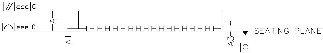
SIDE VIEW
