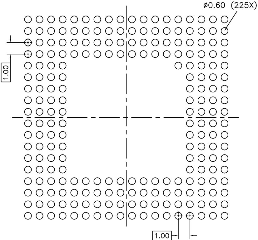
TYPICAL RECOMMENDED LAND PATTERN
