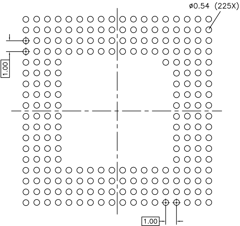
TYPICAL RECOMMENDED STENCIL
