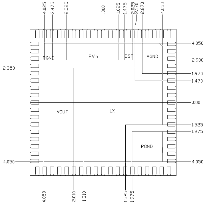
TERMINAL AND PAD EDGE DETAILS
