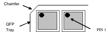
MQFP, LQFP, QFP, T/QFN, LGA (in Trays)
