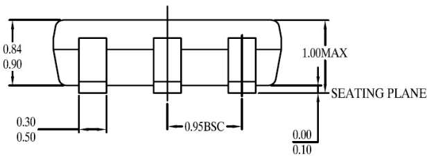
SIDE VIEW - 2
