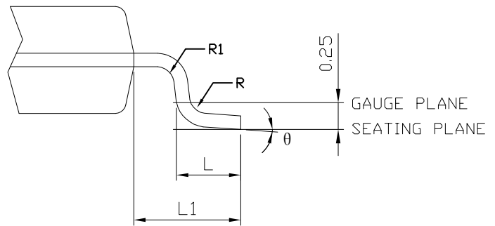
SIDE VIEW - 2
