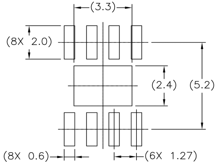
LAND PATTERN RECOMMENDED
