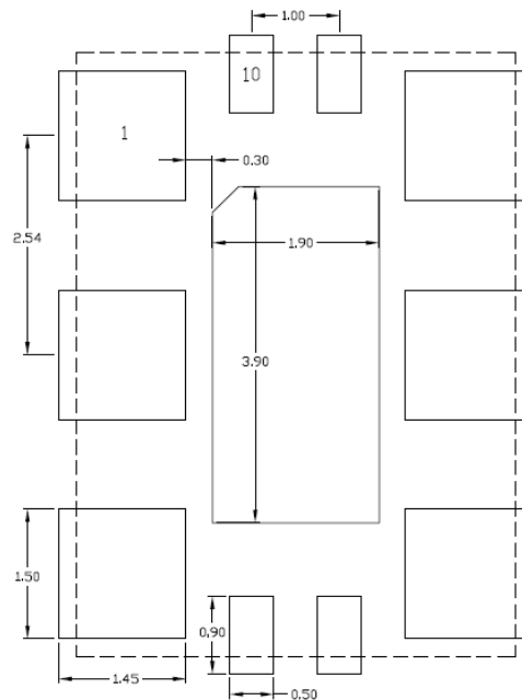
TYPICAL RECOMMENDED LAND PATTERN
